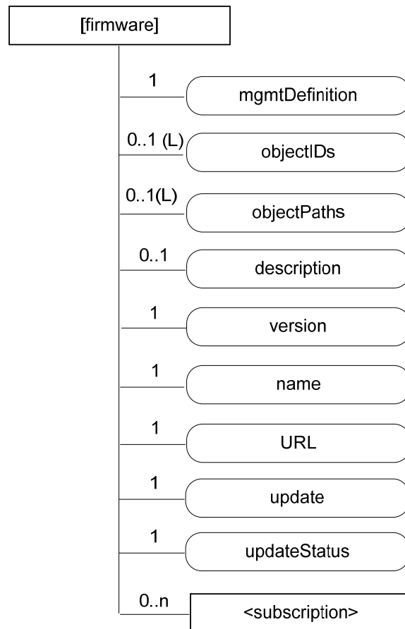
Figure D.2-1: Structure of [firmware] resource
