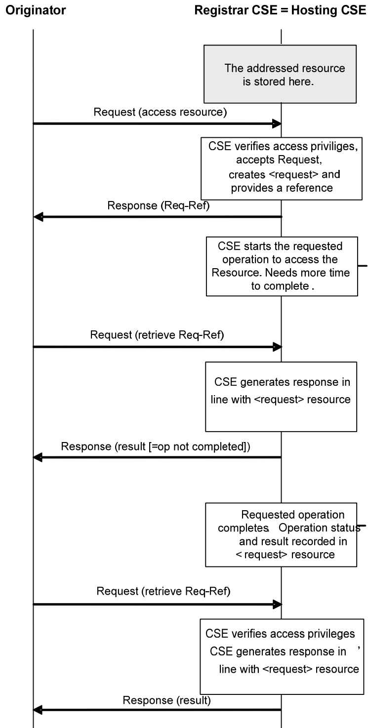
Figure 8.2.2-2: Non-blocking access to resource in synchronous mode (Hosting CSE = Receiver CSE), requested operation completed after the second but before the third request
