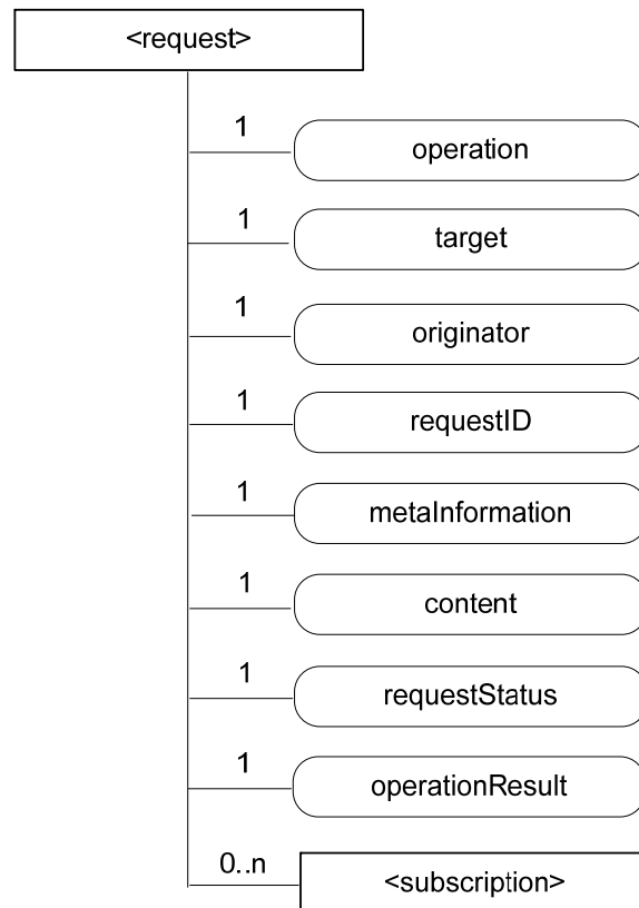
Figure 9.6.12-1: Structure of <request> resource
