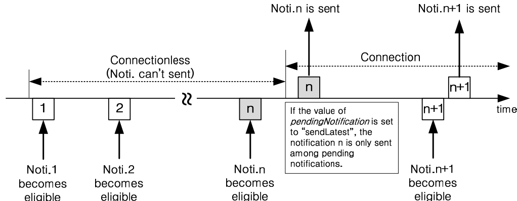
Figure 10.2.12-1: Notification Mechanism when pendingNotification (sendLatest) is used
