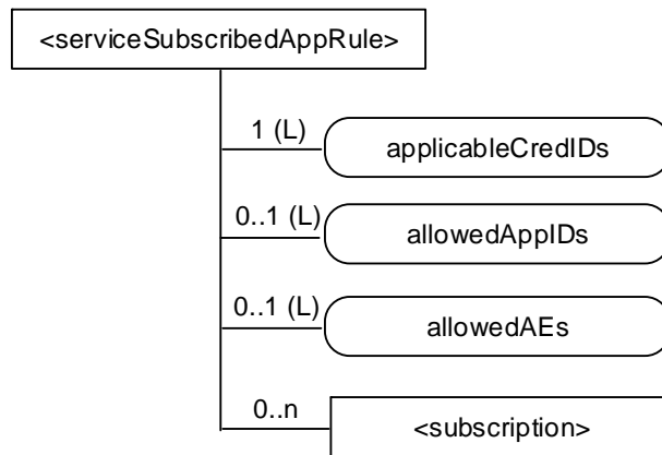
Figure 9.6.29-1: Structure of <serviceSubscribedAppRule> resource
