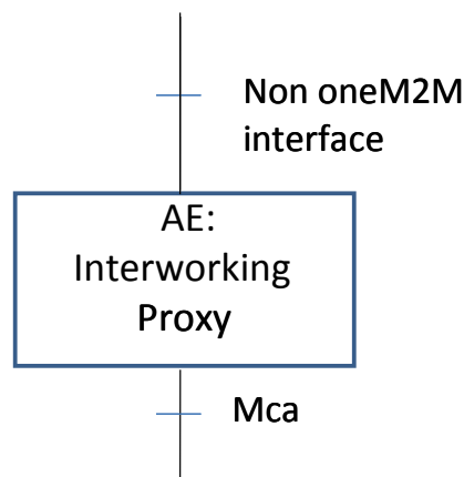
Figure F.2-1: Interworking Proxy
