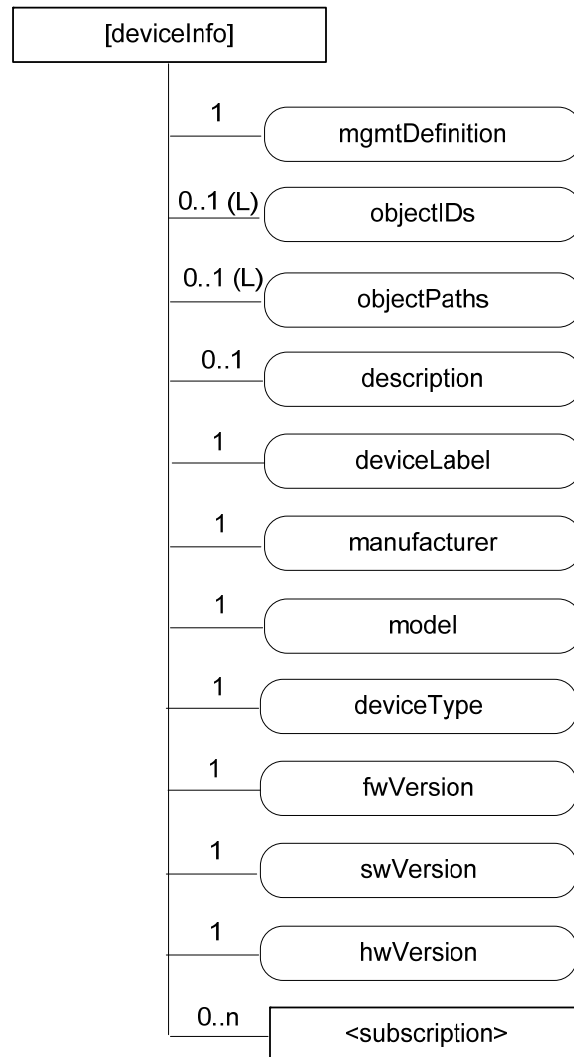
Figure D.8-1: Structure of [deviceInfo] resource
