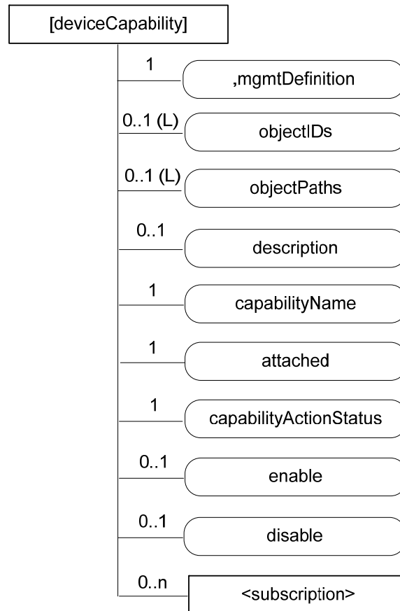
Figure D.9-1: Structure of [deviceCapability] resource
