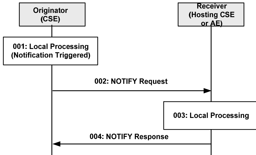
Figure 10.1.5-1: Procedure for NOTIFYing Information
