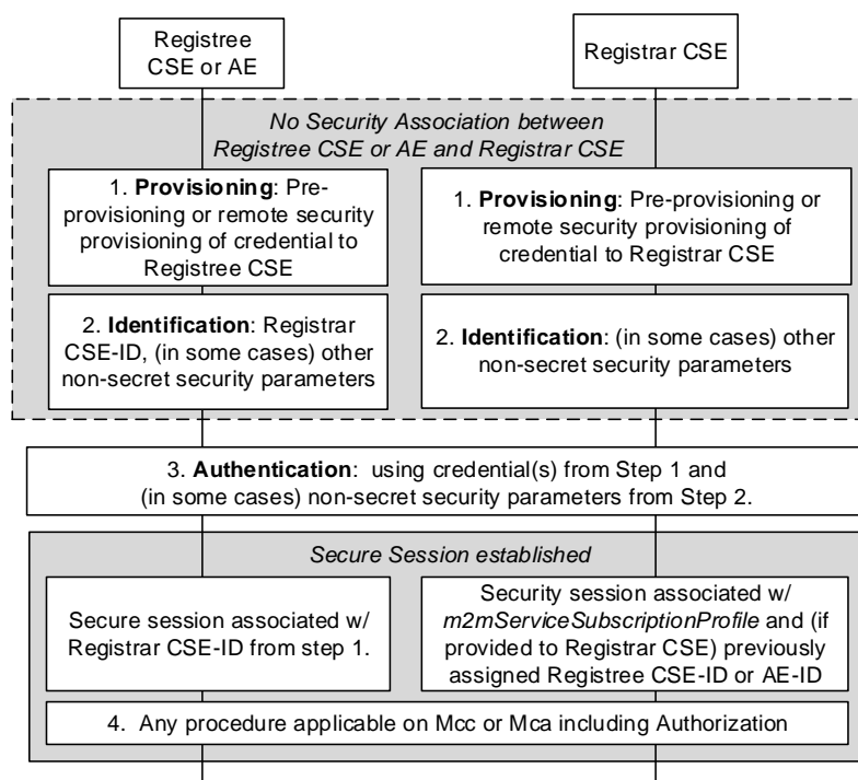
Figure 11.3-1: High Level Procedures on Mcc or Mca
