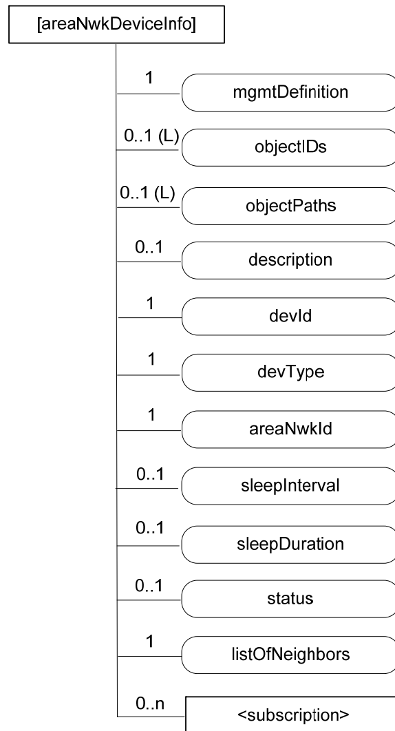
Figure D.6-1: Structure of [areaNwkDeviceInfo] resource
