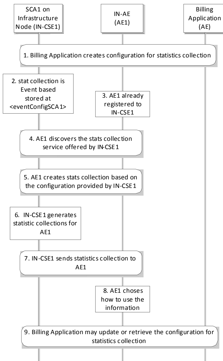
Figure 10.2.15.1-1: Event-based Statistics Collection for Applications © oneM2M Partners Type 1 (ARIB, ATIS, CCSA, ETSI, TTA, TSDSI, TTA, TTC) Page 209 of 310
