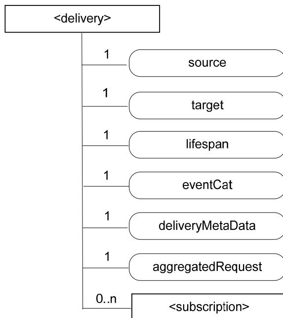
Figure 9.6.11-1: Structure of <delivery> resource
