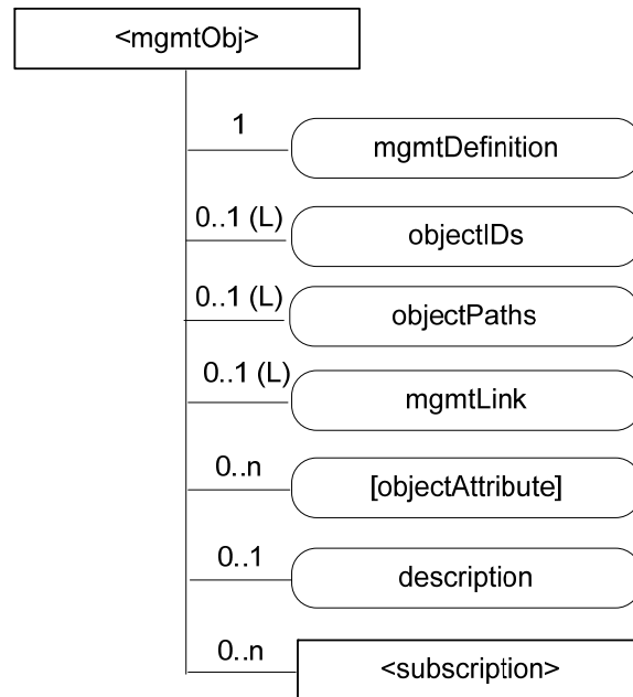
Figure 9.6.15-1: Structure of <mgmtObj> resource
