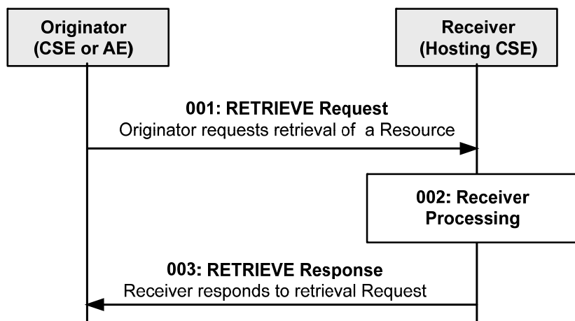
Figure 10.1.2-1: Procedure for RETRIEViNg a Resource
