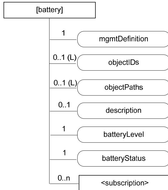
Figure D.7-1: Structure of [battery] resource
