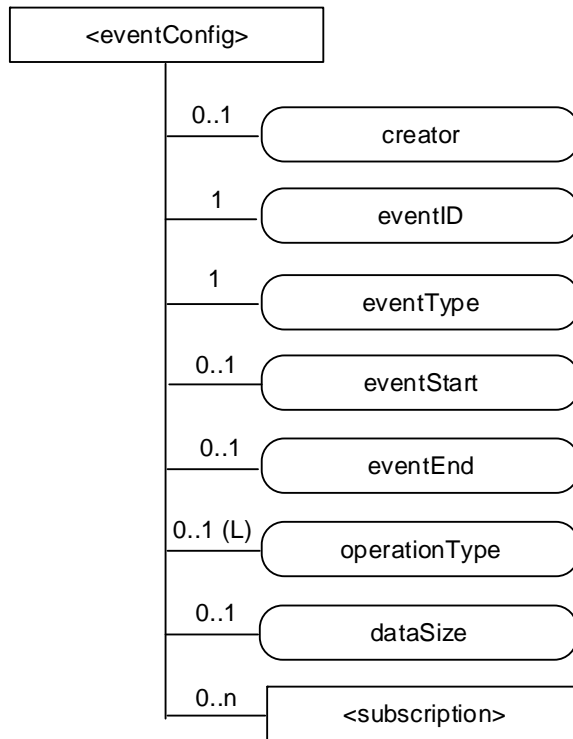
Figure 9.6.24-1: Structure of <eventConfig> resource
