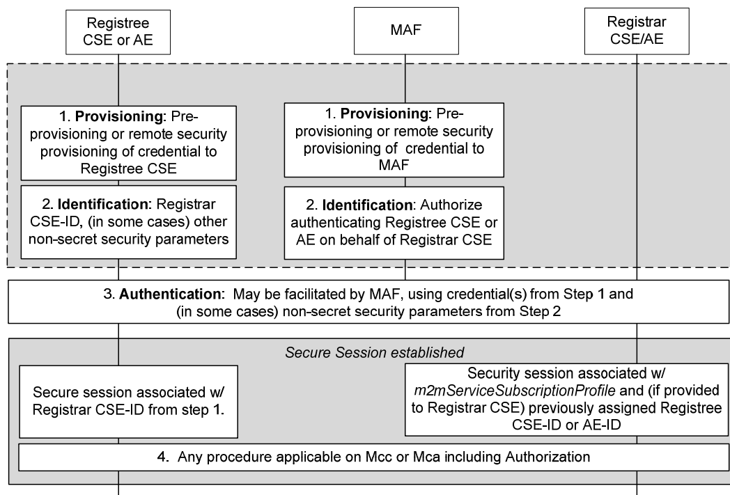
Figure 11.3-2: MAF assisted High Level Procedures on Mcc or Mca
