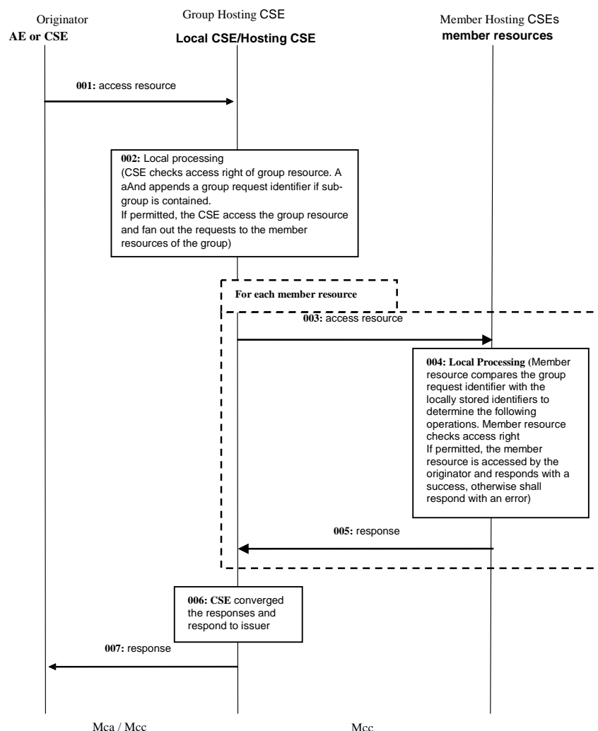
Figure 10.2.7.6-1: Group content management procedures
