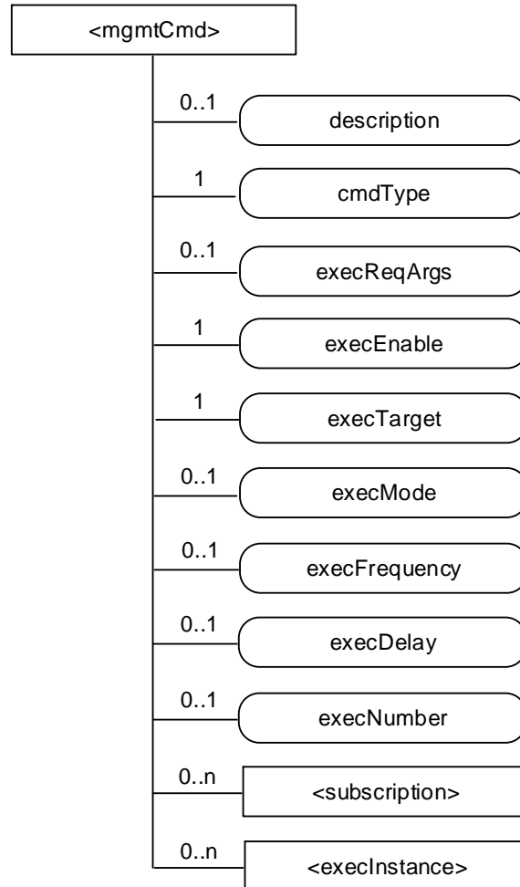
Figure 9.6.16-1: Structure of <mgmtCmd> resource
