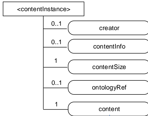
Figure 9.6.7-1: Structure of <contentInstance> resource
