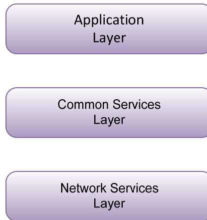
Figure 5.1-1: oneM2M Layered Model
