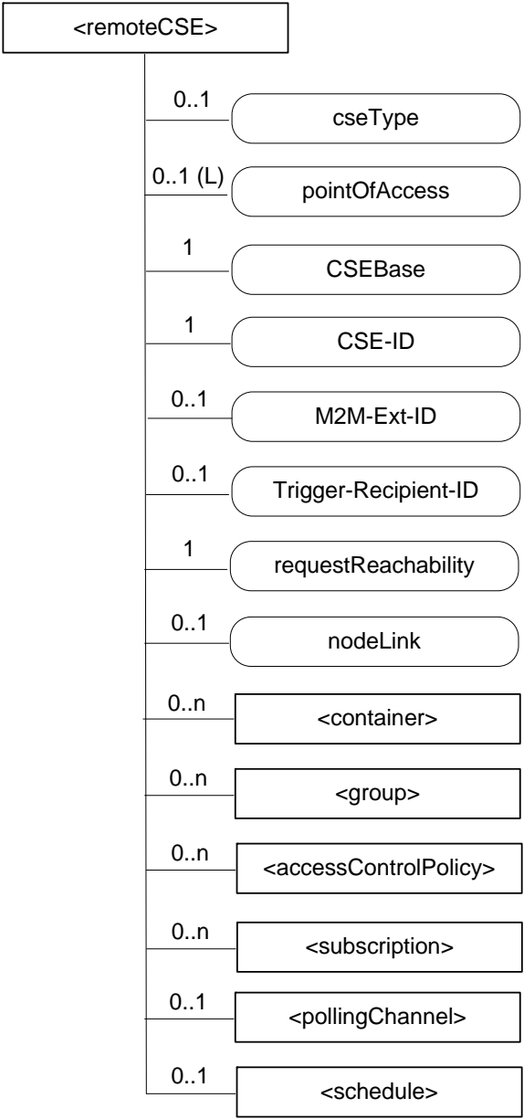
Figure 9.6.4-1: Structure of <remoteCSE> resource
