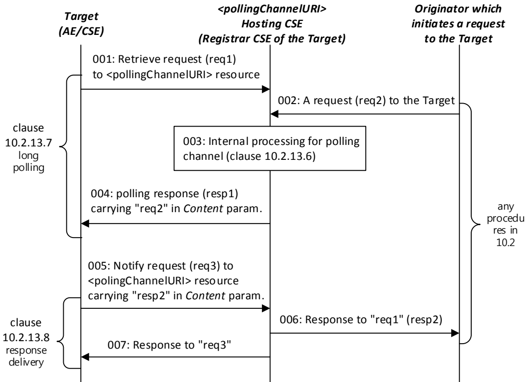
Figure 10.2.13-1: Request/response delivery via polling channel
