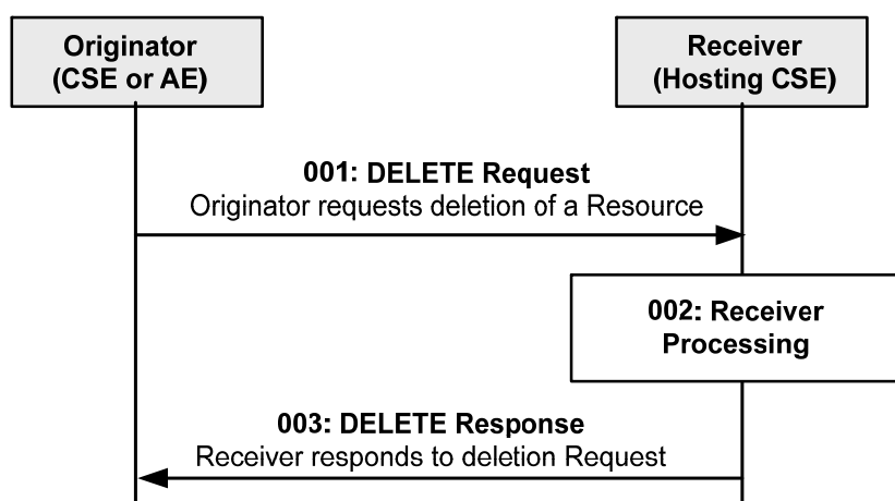
Figure 10.1.4-1: Procedure for DELETING a Resource
