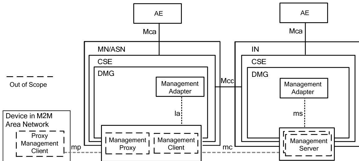
Figure 6.2.4.1.1-1: Device Management Architecture
