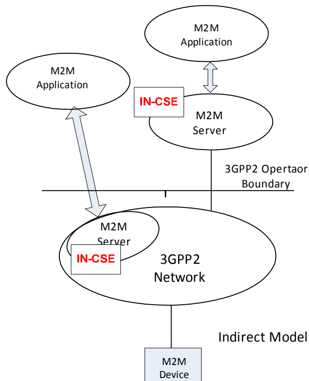
Figure C.2-2: Multiple M2M Applications Using Diverse Communication Models
