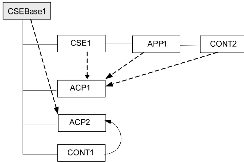
Figure 9.4.1-1: Resource Relationships Example in a CSE
