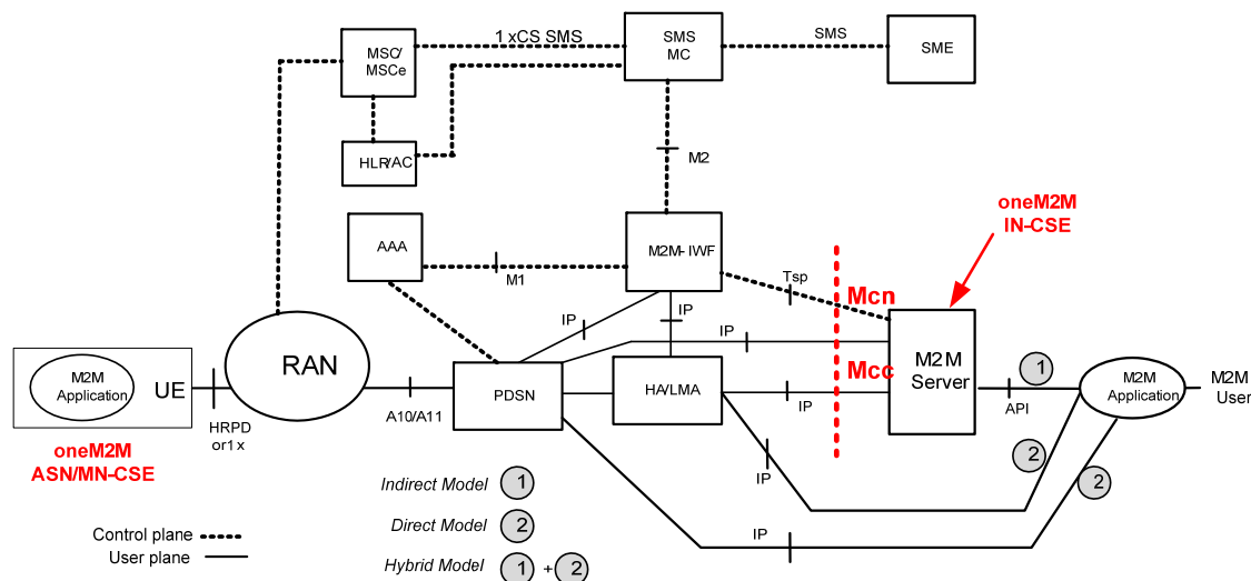
Figure C.3-1: Enhanced 3GPP2 Network Architecture for Supporting M2M
