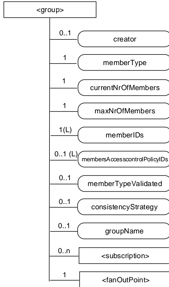
Figure 9.6.13-1: Structure of <group> resource
