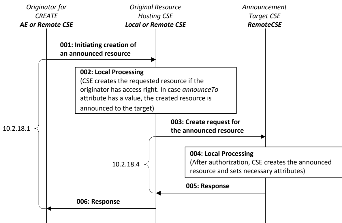
Figure 10.2.18.1-1: Announced resource CREATE procedures
