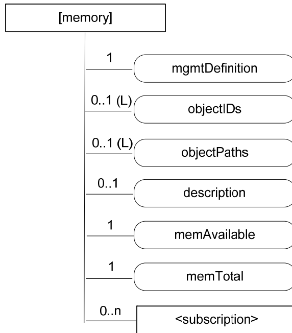
Figure D.4-1: Structure of [memory] resource
