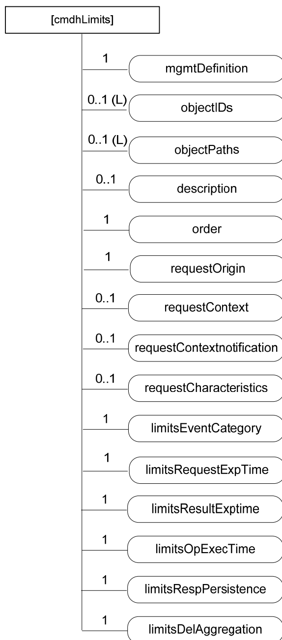
Figure D.12.5-1: Structure of [ cmdhLimits ] resource
