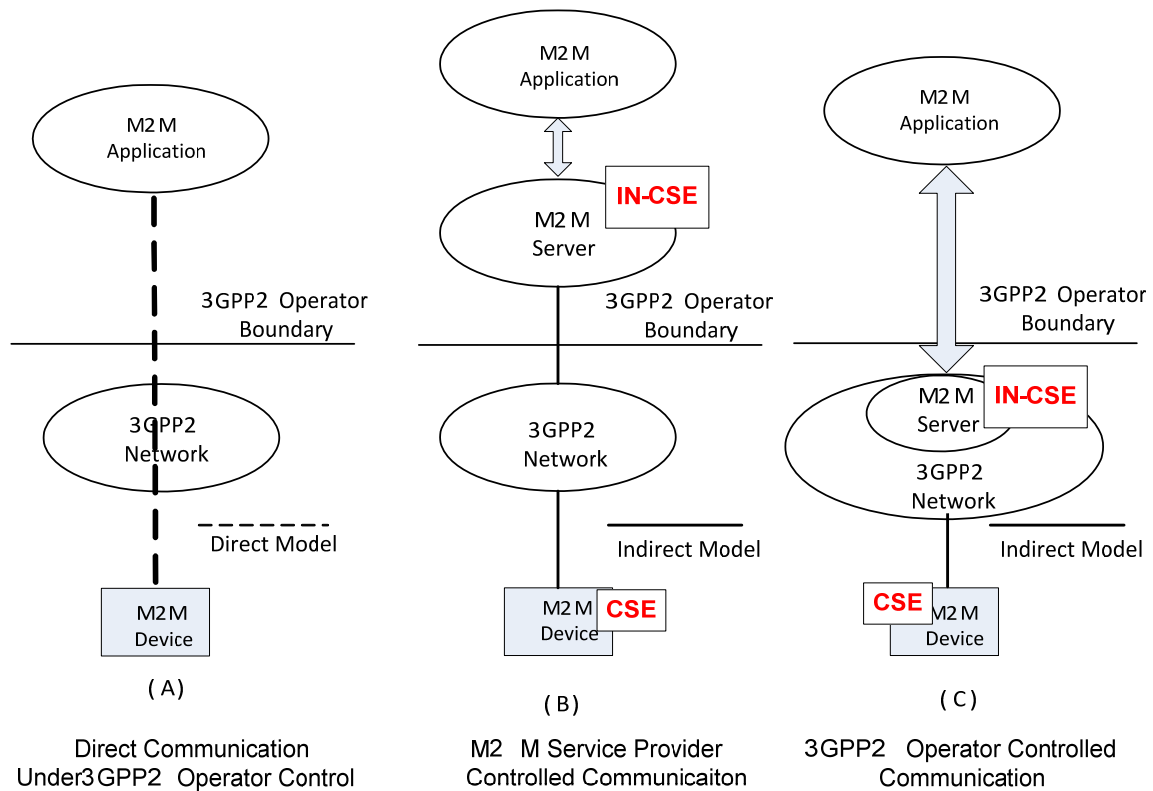
Figure C.2-1: M2M Communication Models
