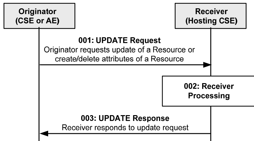
Figure 10.1.3-1: Procedure for UPDATIng a Resource
