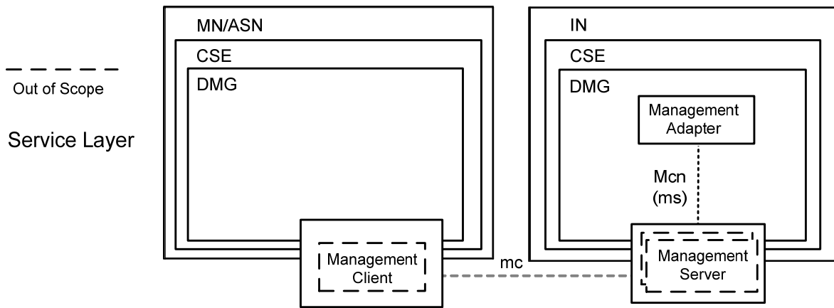
Figure 6.2.4.1.2.1-2: Management Server in M2M Service Layer
