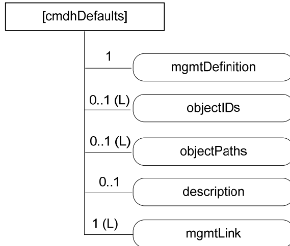
Figure D.12.2-1: Structure of [cmdhDefaults] resource
