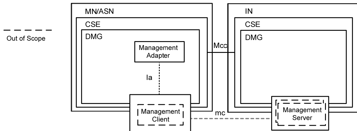
Figure 6.2.4.1.3.1-1: Management Client Interaction using "la" interface
