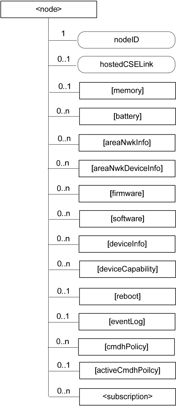
Figure 9.6.18-2: Structure of <node> resource
