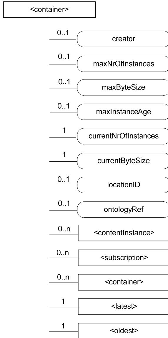
Figure 9.6.6-1: Structure of <container> resource
