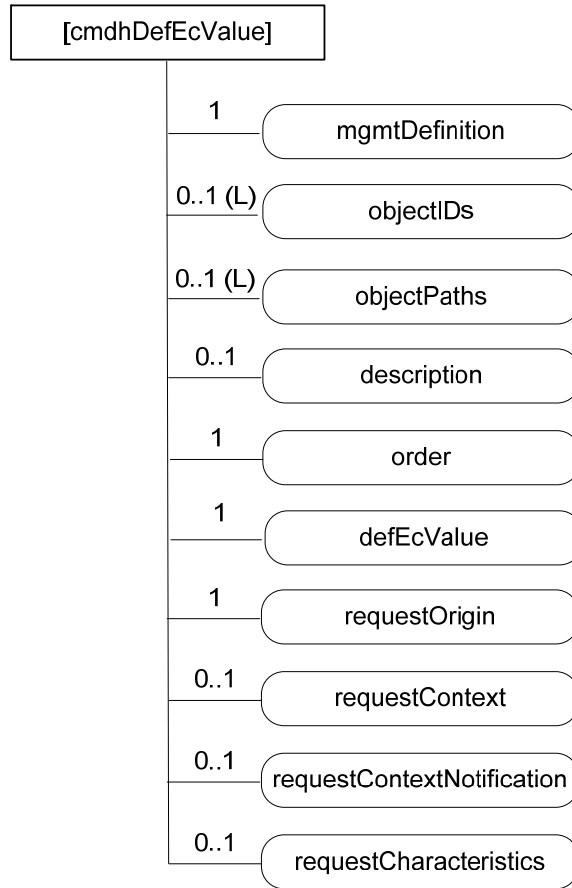
Figure D.12.3-1: Structure of [cmdhDefEcValue] resource
