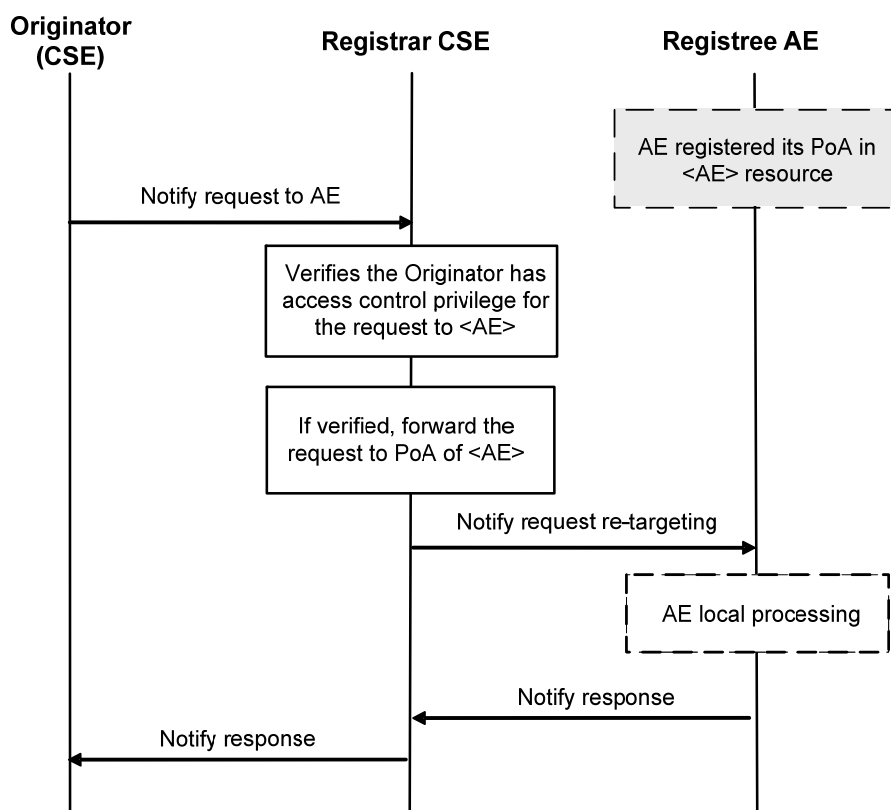
Figure 9.3.2.3-1: Re-targeting a notification request to an AE
