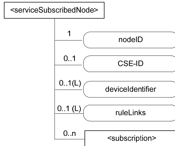
Figure 9.6.20-1: Structure of <serviceSubscribedNode> resource
