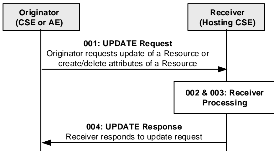
Figure 6.4.2.5-1: Procedure for UPDATing a Resource (TS-0001 Clause 10)
