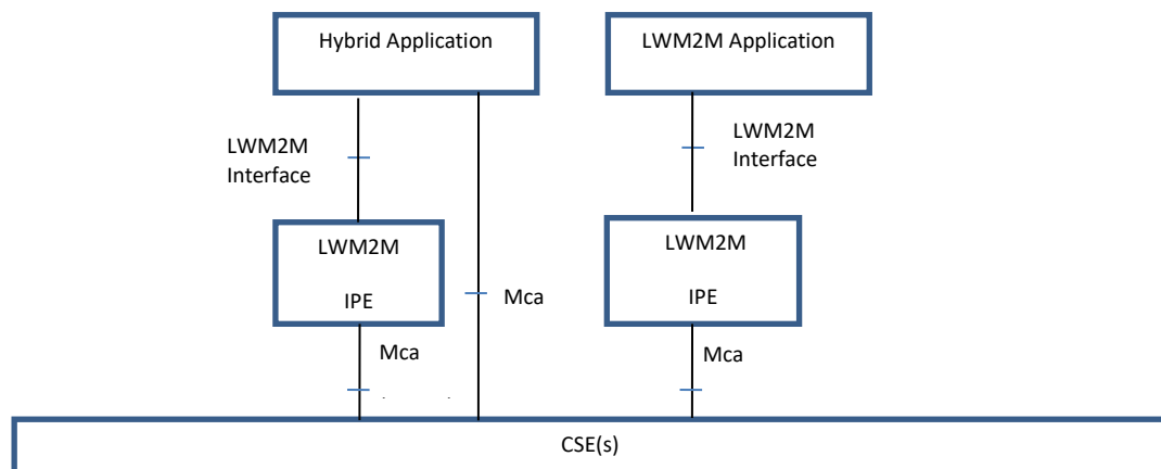
Figure 5.1-1: LWM2M Interworking Scenarios
