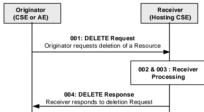
Figure 6.4.2.6-1: Procedure for Deleting a resource (oneM2M TS-0001 [2], clause 10)
