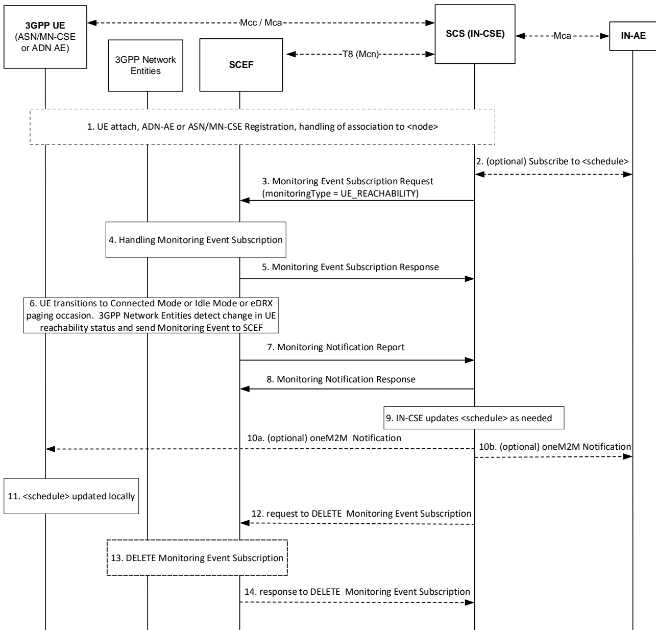
Figure 7.4.1 -1: Procedure for UE Reachability monitoring
