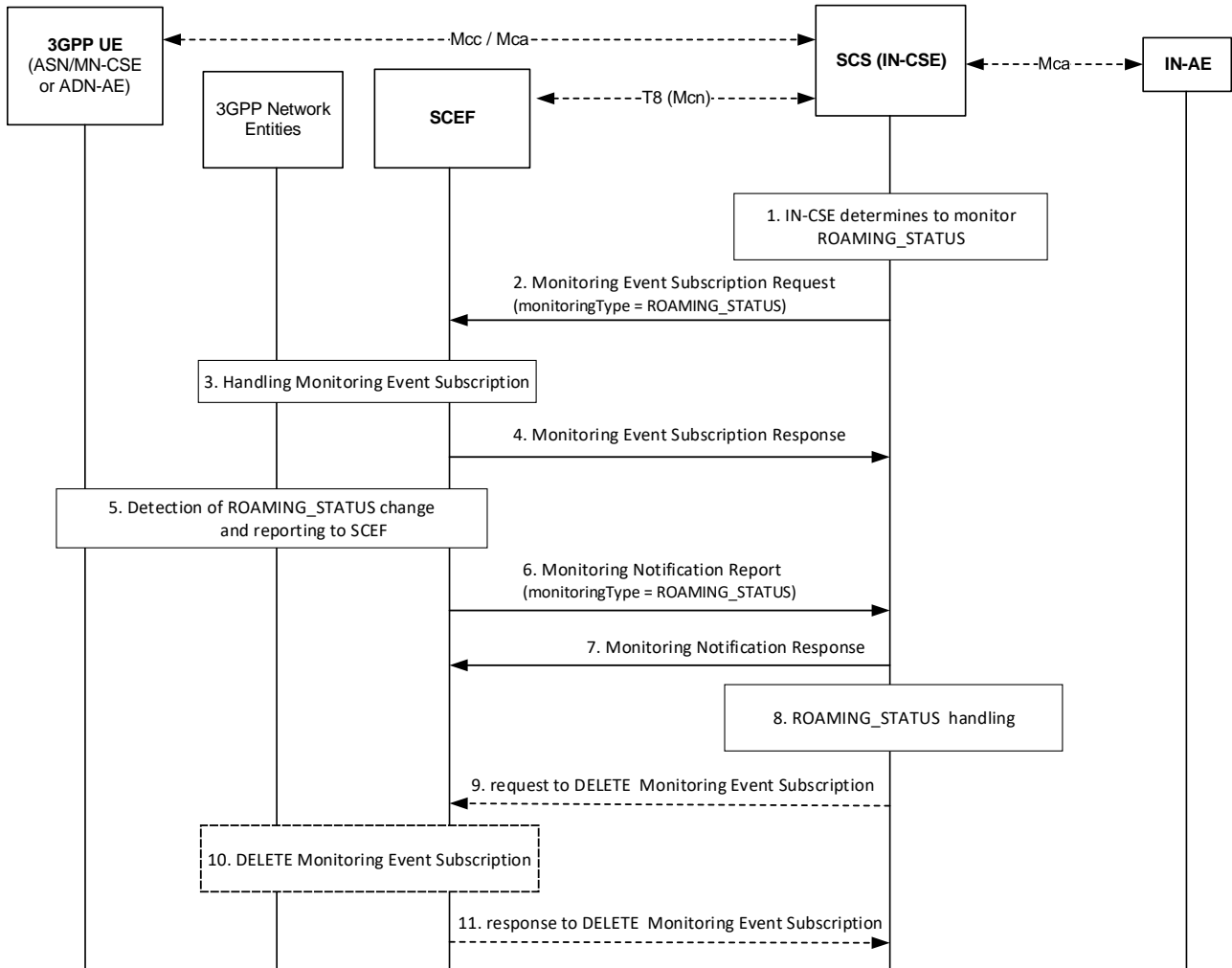
Figure 7.4.6-1: Request for Roaming Status Indications
