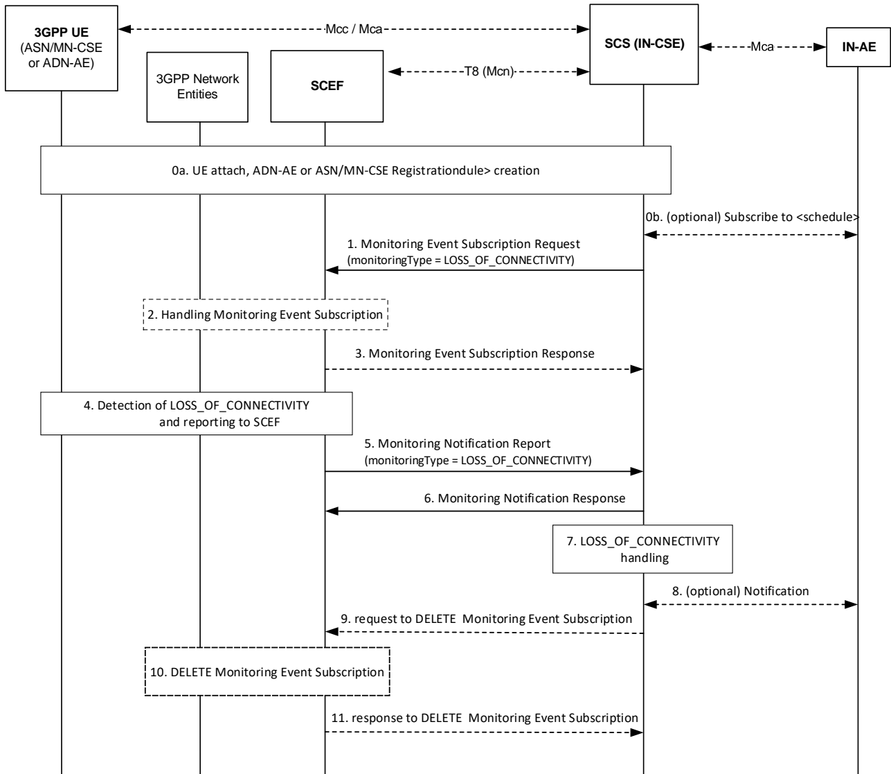
Figure 7.4.4-1: Loss of Connectivity monitoring
