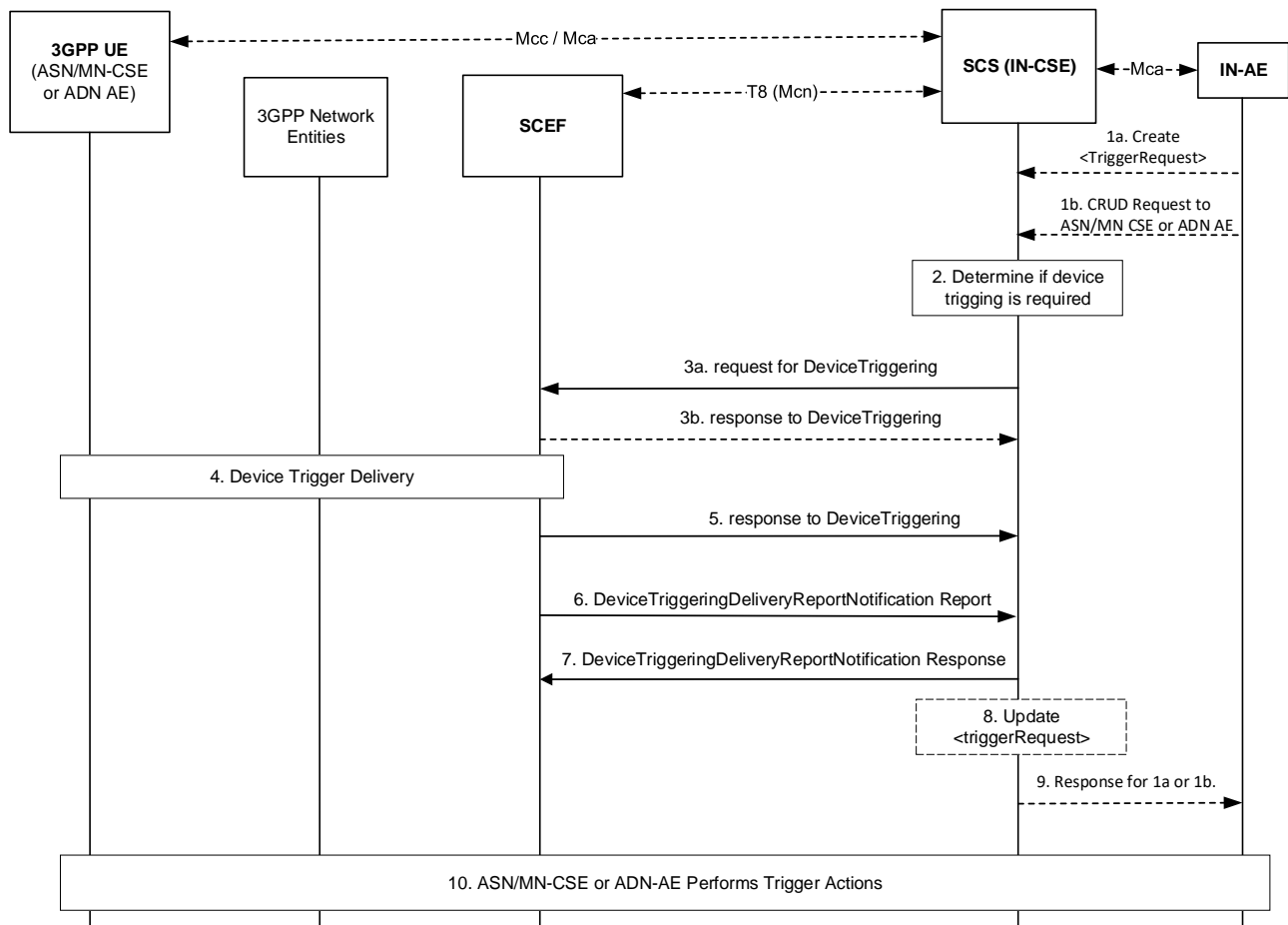
Figure 7.5.1-1: General Procedure for Device Triggering
