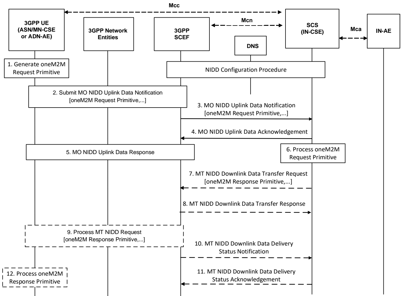
Figure 7.1.1.3-1: SCEF-based Mobile Originated NIDD
