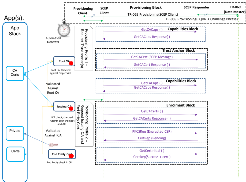
Figure M.2-1: SCEP certificate provisioning procedure
