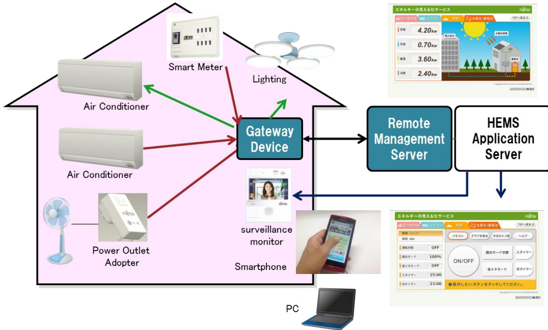
2220 2221 Figure 9-3 Home Energy Management System High Level Illustration 2222
