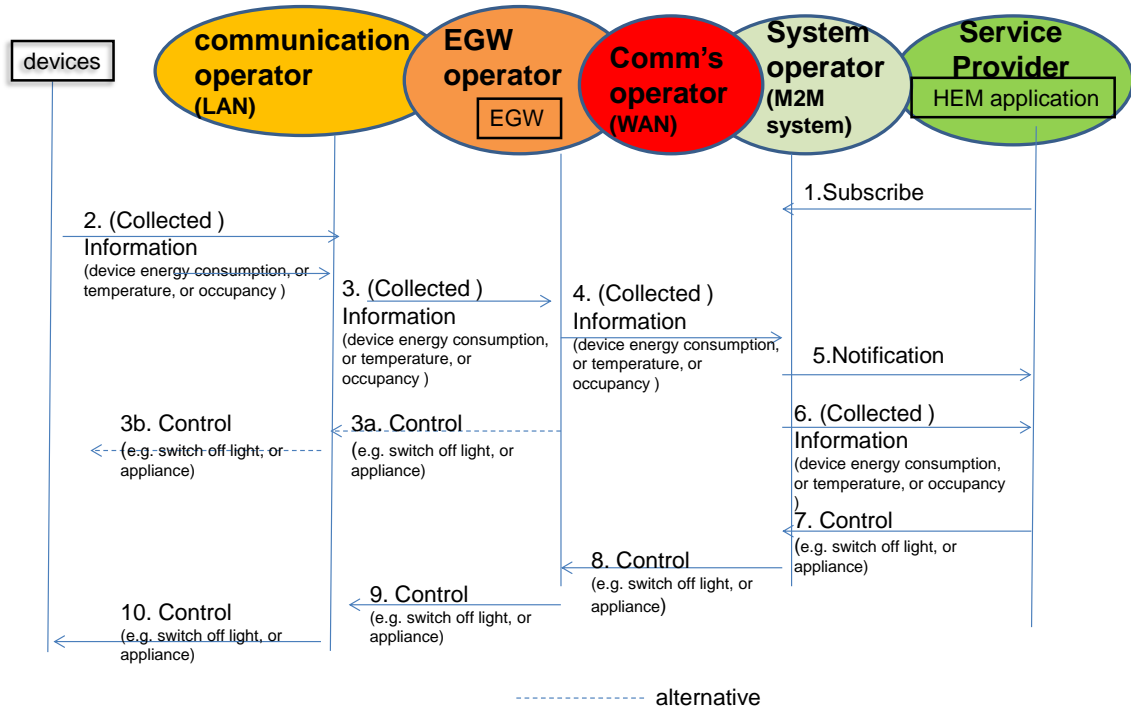
Figure 9-1 Home Energy Management Normal Flow
