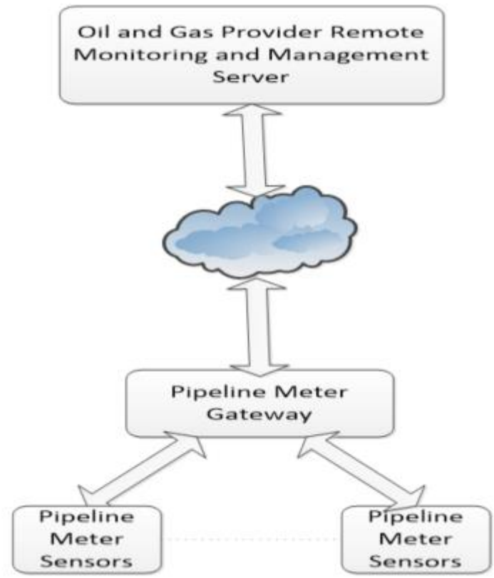
536 537 Figure 5-13 High Level Illustration - Oil and Gas Pipeline Gateway 538
